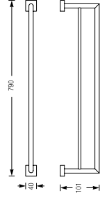
DOUBLE BATH TOWEL SHELF WBBA100177CP
