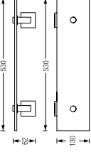
GLASS SHELF WBBA100172CP
