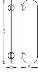
GLASS SHELF WITH TEMPERED GLASS WBBA100124CP
