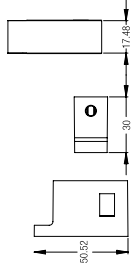
TOWEL RING, 30x12.5CM WBBA1.00255CP
